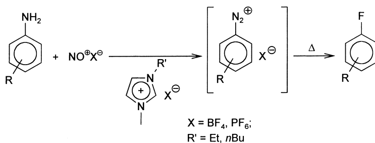
Scheme 2. One-pot diazotization-fluorodediazotization in ionic liquid solvents.
